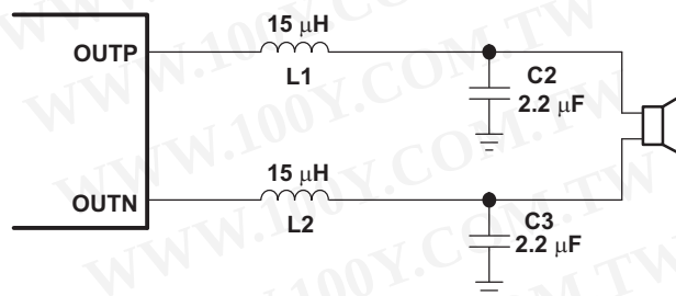
Figure 42. Typical LC Output Filter, Cutoff Frequency of 27 kHz, Speaker Impedance = 4 Ω
