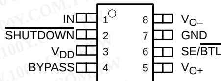
DGN PACKAGE (TOP VIEW)
