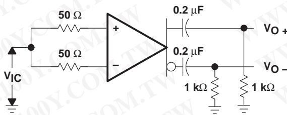
Figure 3. Test Circuit
