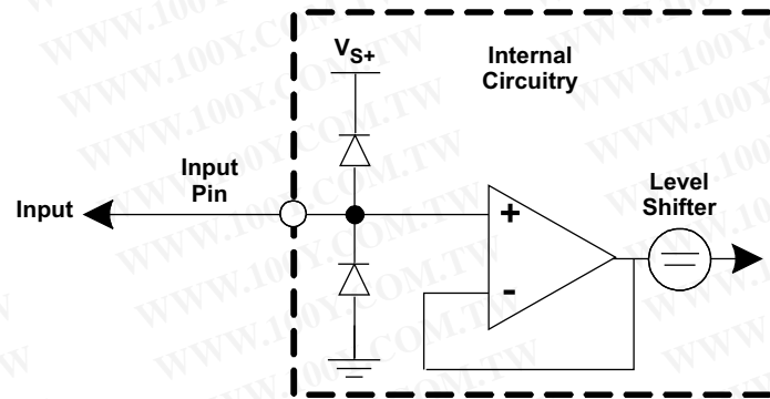
Figure 61. Equivalent DC + 250 mV Input Mode Circuit
