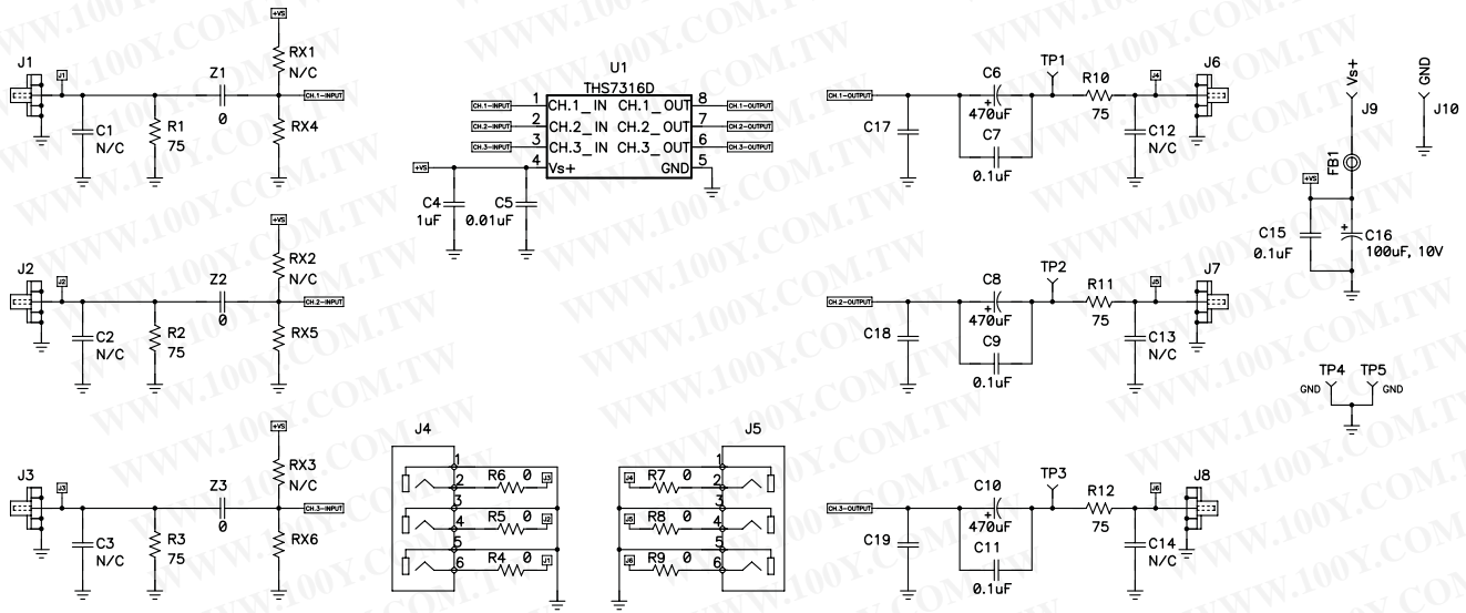
Figure 33. THS7316D EVM
