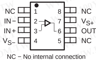
THS4601 D AND DDA PACKAGE (TOP VIEW)
