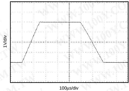
LARGE-SIGNAL STEP RESPONSE G = 1 , R_L = 1\text{M}\Omega
