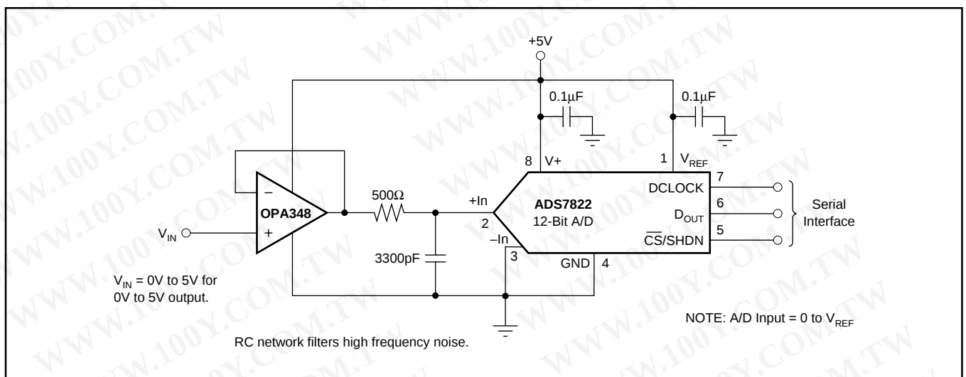
FIGURE 7. OPA348 in Noninverting Configuration Driving ADS7822.
