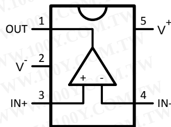
Figure 1. 5-Pin SC70 Top View
