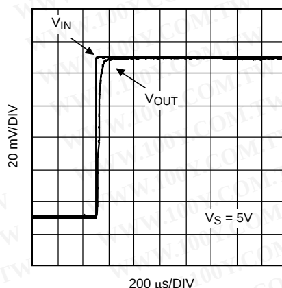
Figure 67. Step Response
