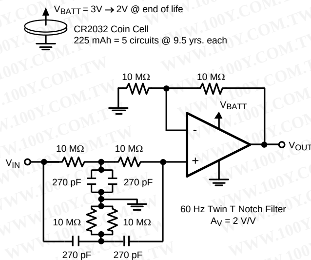
Figure 62. 60 Hz Notch Filter
