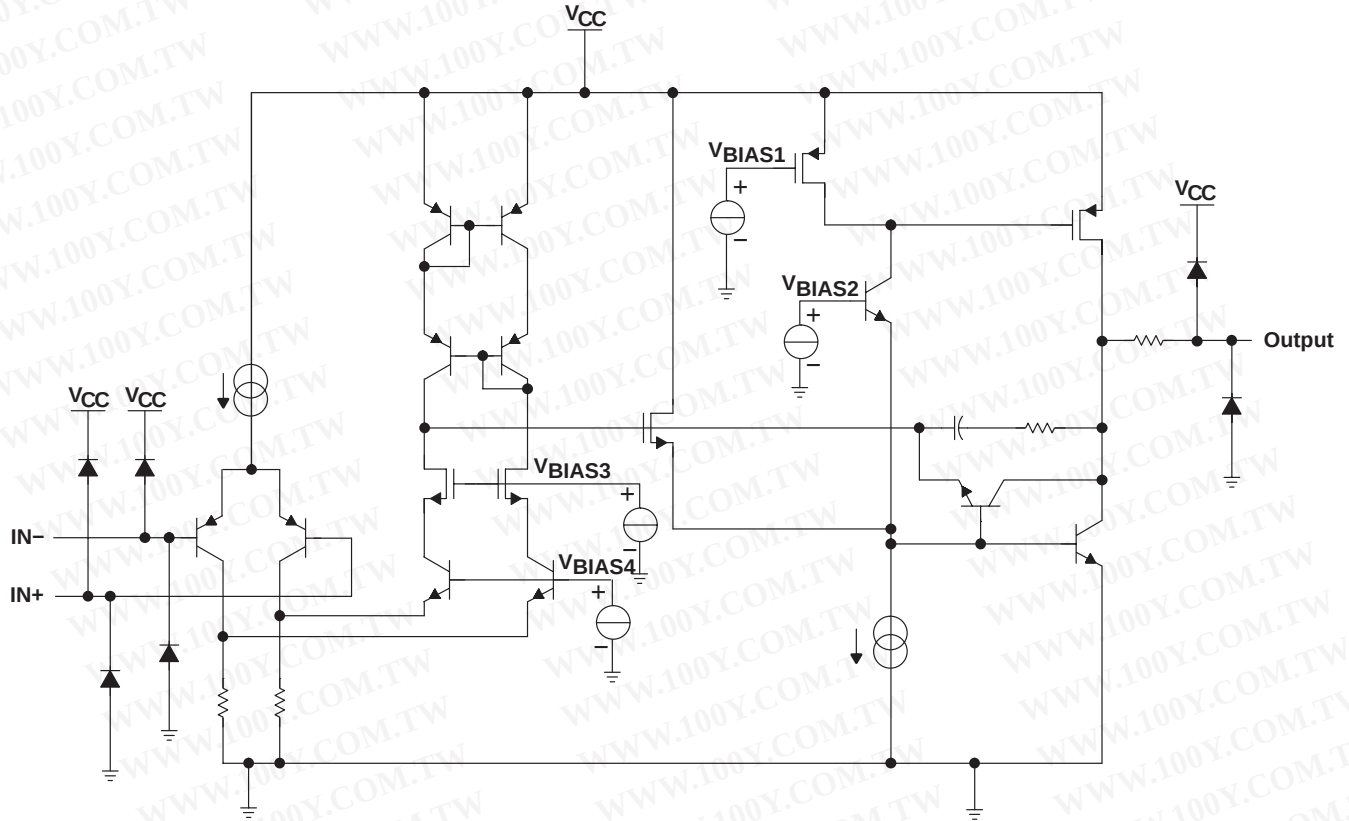
LPV324 simplified schematic
