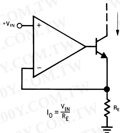
Figure 69. High Compliance Current Sink
