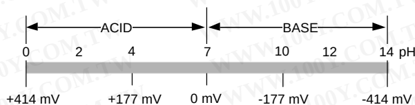
Figure 54. Output Voltage of a pH Electrode
