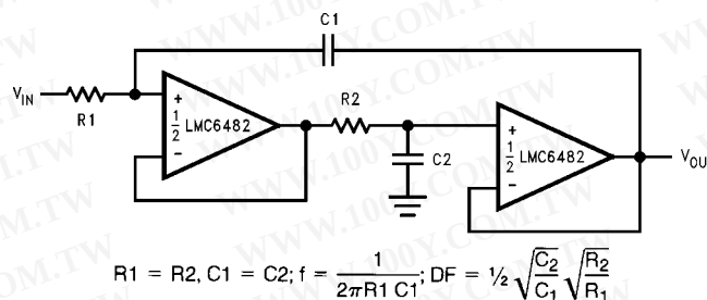
Figure 82. Rail-to-Rail Single Supply Low Pass Filter
