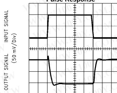
Inverting Small Signal Pulse Response
