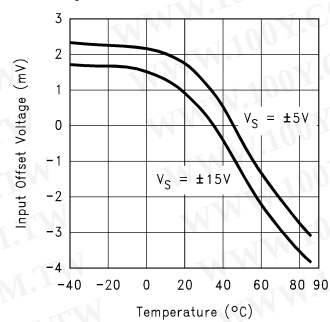
Input Offset Voltage vs Temperature
