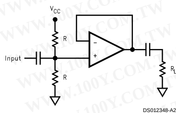
(e) A_v = +1 , V_S = +5\text{V} , Single Supply Operation
