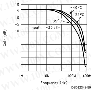
Closed Loop Frequency Response vs Temperature V_S = \pm 5\text{V} , A_V = +2 , R_L = 100\Omega
