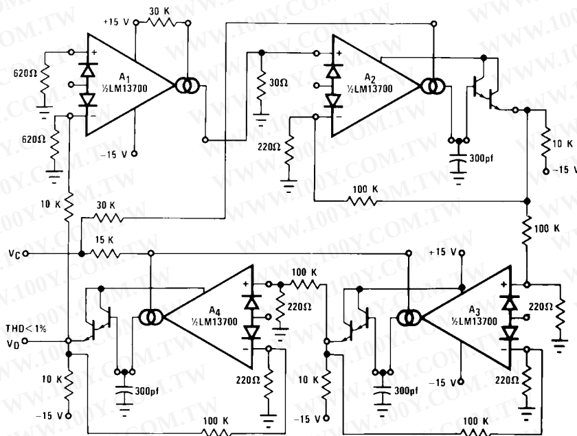
Figure 38. Sinusoidal VCO
