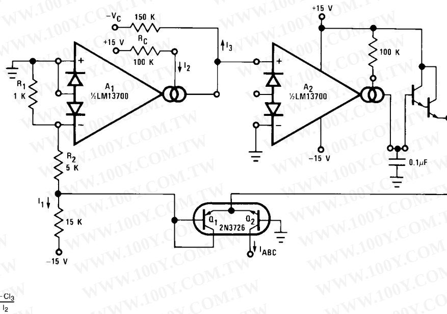
Figure 51. Logarithmic Current Source
