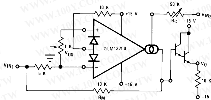
Figure 27. Four-Quadrant Multiplier
