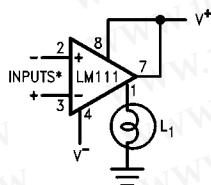
Figure 46. Driving Ground-Referenced Load
