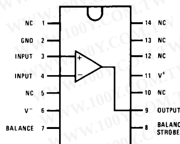
Figure 61. 14-Pin CDIP (See J Package) 14-Pin PDIP (See NFF Package)
