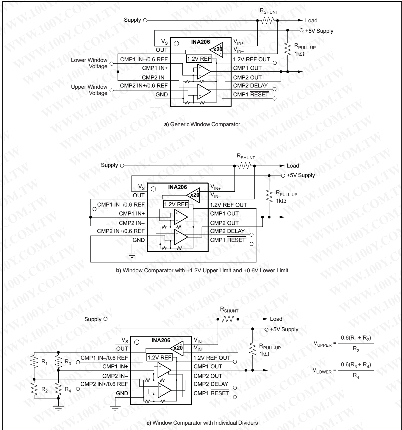
Figure 41. Using the INA206, INA207, and INA208 as Window Comparators
