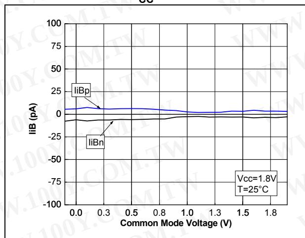
Figure 18. Input bias current vs. common mode at V_{CC} = 1.8 V
