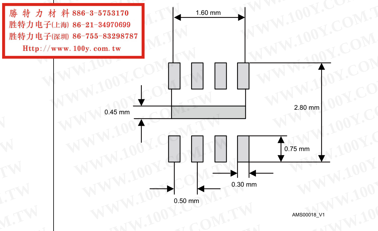
Figure 55. DFN8 2x2 footprint recommendation
