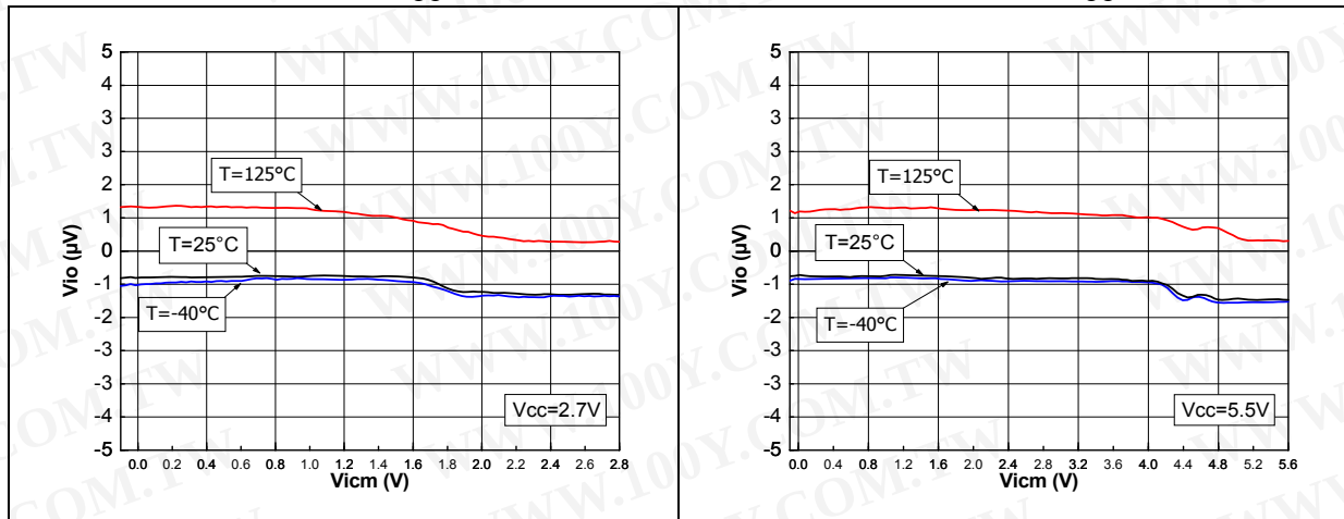
Figure 10. Input offset voltage vs. input common mode at V_{CC} = 2.7\text{ V}
