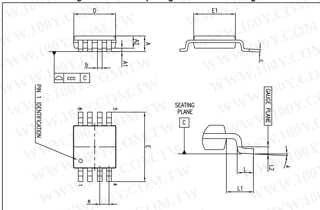
Figure 56. MiniSO-8 package mechanical drawing
