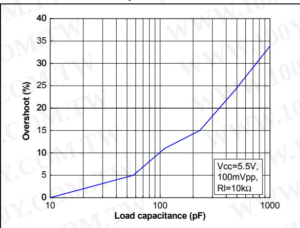
Figure 29. Output overshoot vs. load capacitance
