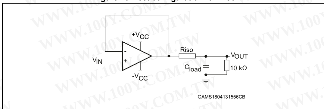
Figure 45. Test configuration for Riso
