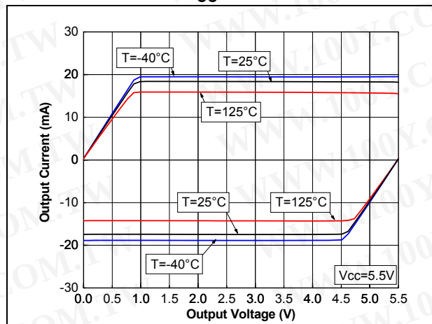
Figure 16. Output current vs. output voltage at V_{CC} = 5.5 V
