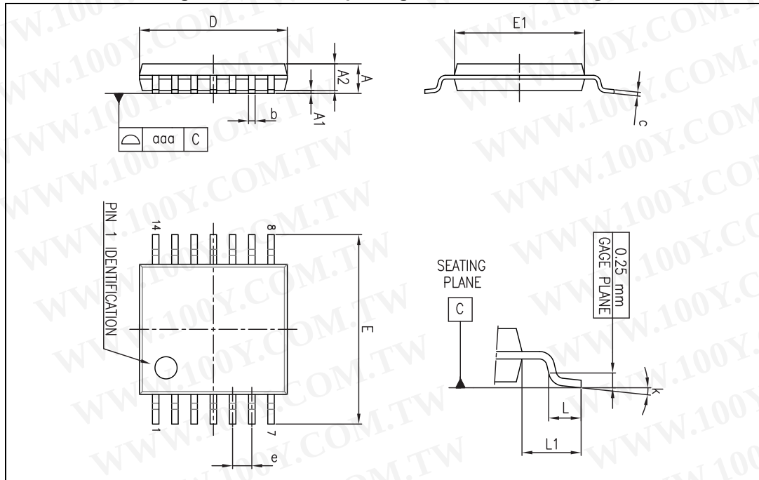
Figure 59. TSSOP14 package mechanical drawing
