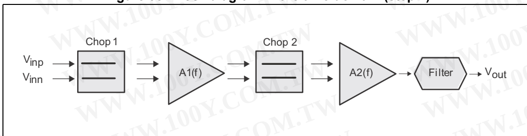
Figure 38. Block diagram in the time domain (step 1)
