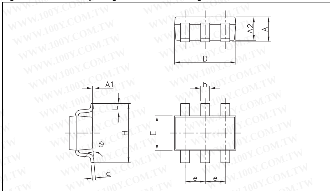
Figure 35. SOT23-6L package mechanical drawing
