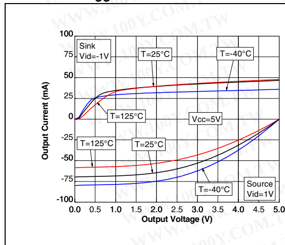
Figure 6. Output current vs. output voltage at V_{CC} = 5\text{ V}
