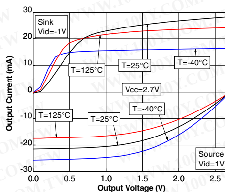
Figure 5. Output current vs. output voltage at V_{CC} = 2.7\text{ V}
