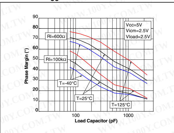
Figure 11. Phase margin vs. load capacitor at V_{CC} = 5\text{ V}
