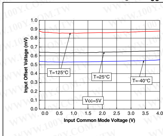
Figure 4. Input offset voltage vs. input common mode voltage at V_{CC} = 5\text{ V}
