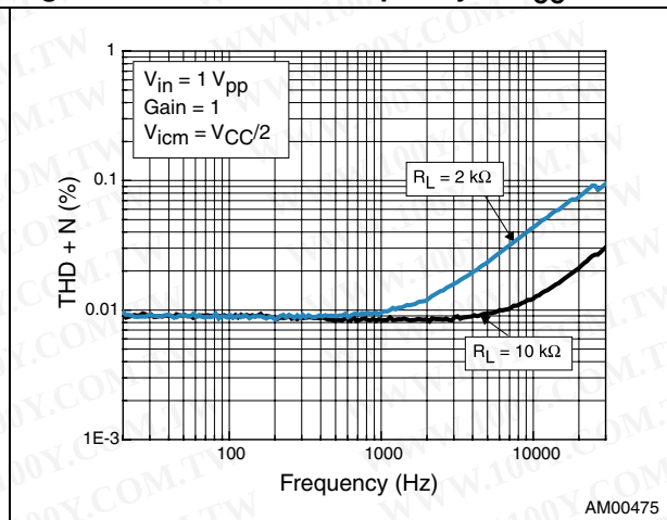
Figure 16. THD+N vs. frequency at V_{CC} = 2.7\text{ V} Figure 17. THD+N vs. frequency at V_{CC} = 5.5\text{ V}
