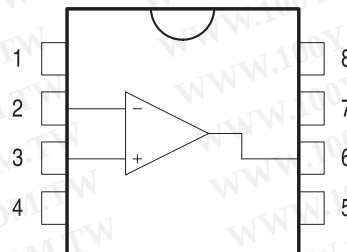
Pin connections (top view)
