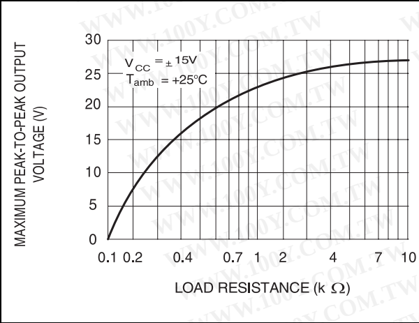
Figure 7. Maximum peak-to-peak output voltage versus load resistance
