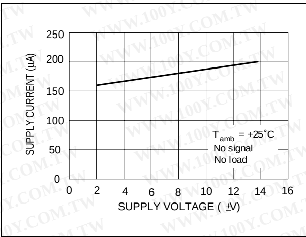
Figure 8. Supply current per amplifier versus supply voltage
