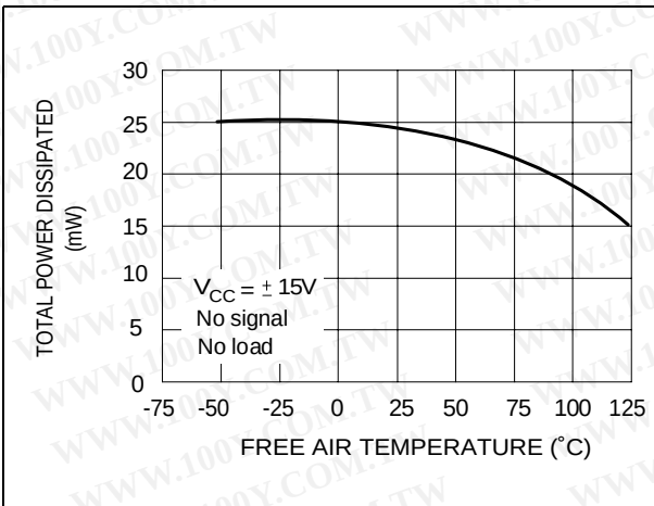
Figure 10. Total power dissipated versus free air temperature
