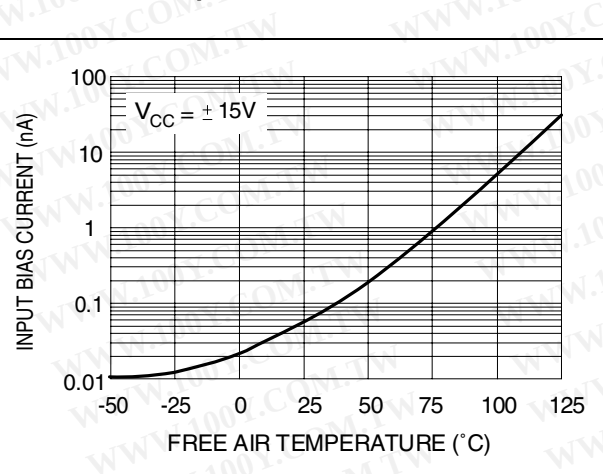
Figure 14. Input bias current versus free air temperature
