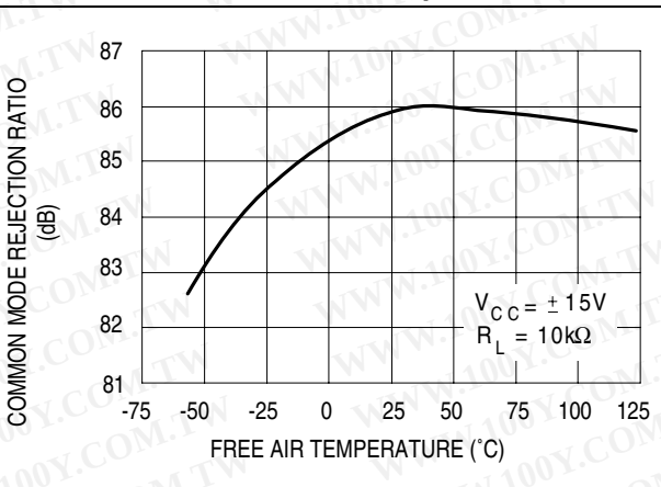
Figure 12. Common mode rejection ratio versus free air temperature
