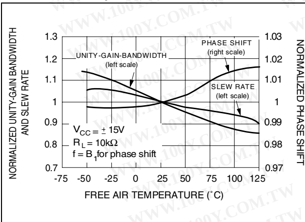
Figure 13. Normalized unity gain bandwidth, slew rate, and phase shift versus temperature
