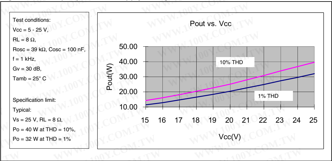
Figure 11. Output power vs. supply voltage
