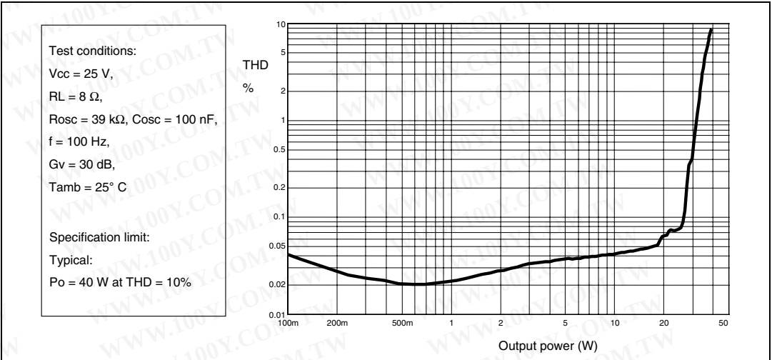
Figure 13. THD vs. output (100 Hz)
