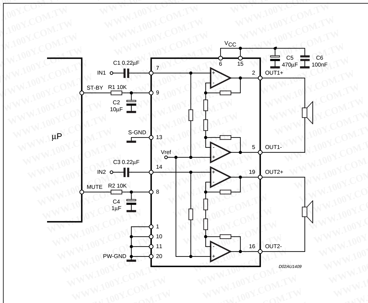
Figure 1. Microprocessor Application
