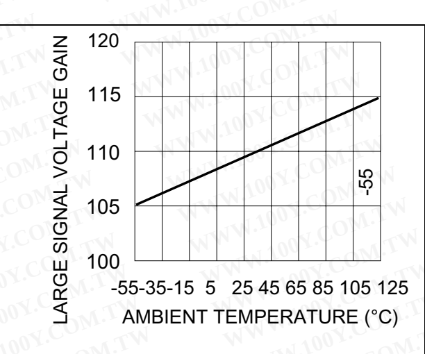
Figure 18. Large signal voltage gain
