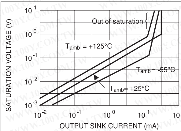
Figure 4. Output saturation voltage vs. output current
