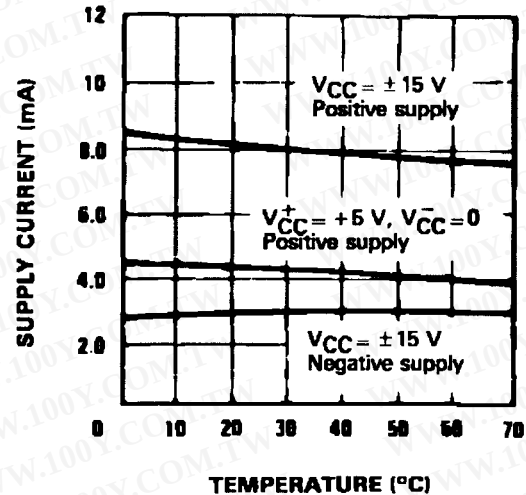
SUPPLY CURRENT
