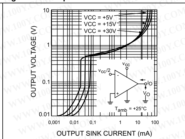
Figure 7. Output characteristics
