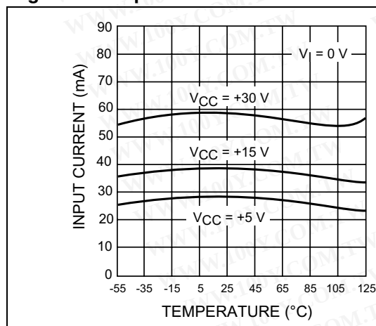
Figure 6. Input current
