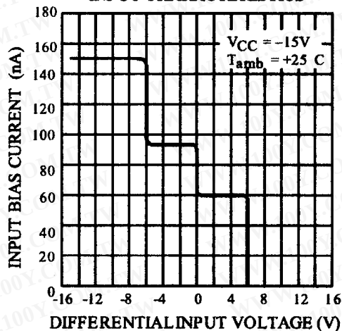
INPUT CHARACTERISTICS
