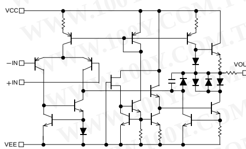
Fig. 225 Simplified schematic (BA14741)
