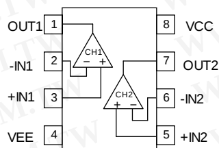
SSOP-B8
