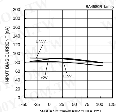
Fig. 100 Input Bias Current – Ambient Temperature (Vicm=0[V], Vout=0[V])
