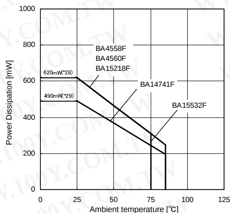
(b)BA4558/BA4560/BA15218/BA14741/BA15532 family
