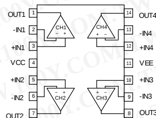
SOP14
