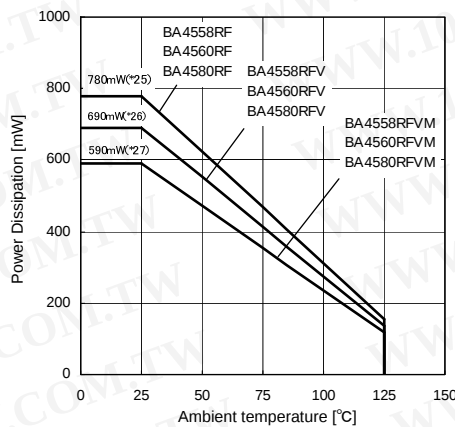
(a)BA4558R/BA4560R/BA4580R family
