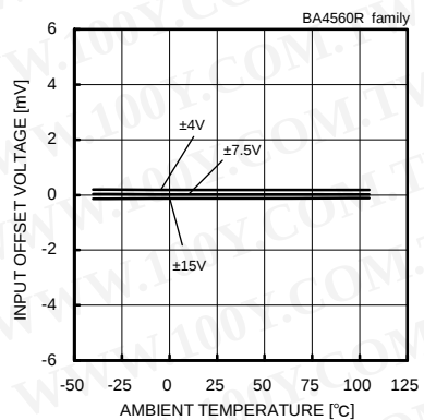
Fig. 76 Input Offset Voltage – Ambient Temperature (Vicm=0[V], Vout=0[V])
