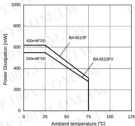
(c)BA4510 family
