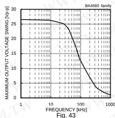
Fig. 43 Maximum Output Voltage Swing – Frequency ( V_{CC}/V_{EE}=+15[V]/-15[V] , R_L=2[k\Omega] , T_a=25[^\circ C] )
