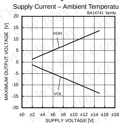
Fig. 138 Maximum Output Voltage – Supply Voltage (RL=2[kΩ], Ta=25[°C])
