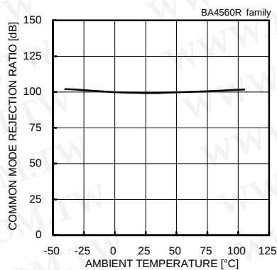
Fig. 82 Common Mode Rejection Ratio – Ambient Temperature ( V_{CC}/V_{EE}=+15[V]/-15[V] , V_{cm}=-12[V] to +12[V] )
