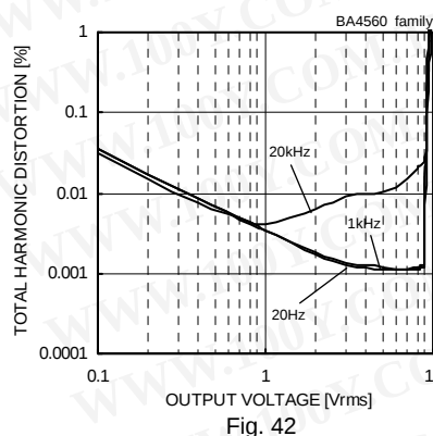
Fig. 42 Total Harmonic Distortion – Output Voltage ( V_{CC}/V_{EE}=+15[V]/-15[V] , A_v=20[dB] , R_L=2[k\Omega] , 80[kHz] -LFP, T_a=25[^\circ C] )
