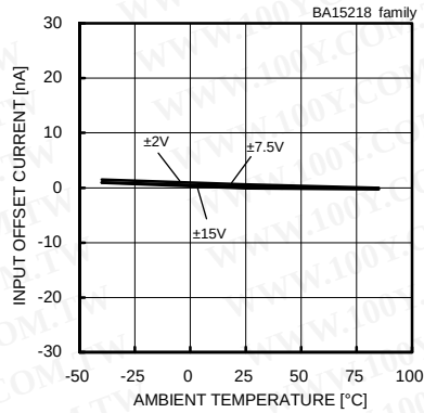
Fig. 212 Input Offset Current - Ambient Temperature ( V_{icm}=0[V] , V_{out}=0[V] )
