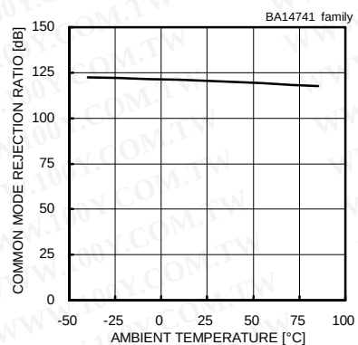
Fig. 236 Common Mode Rejection Ratio - Ambient Temperature ( V_{CC}/V_{EE}=+15[V]/-15[V] , V_{icm}=-12[V] to +12[V] )
