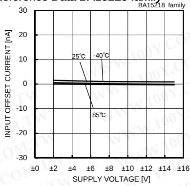
Fig. 211 Input Offset Current - Supply Voltage ( V_{icm}=0[V] , V_{out}=0[V] )
