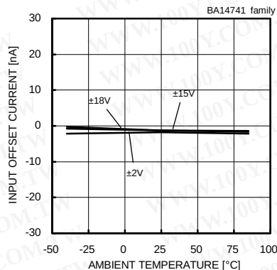
Fig. 234 Input Offset Current - Ambient Temperature ( V_{icm}=0[V] , V_{out}=0[V] )
