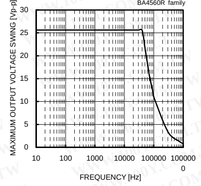
Fig. 87 Maximum Output Voltage Swing - Frequency ( V_{CC}/V_{EE}=+15[V]/-15[V] , R_L=2[k\Omega] , T_a=25[^\circ C] )
