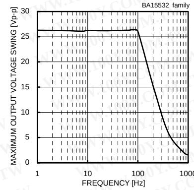
Fig. 263 Maximum Output Voltage Swing - Frequency ( V_{CC}/V_{EE}=+15[V]/-15[V] , R_L=600[\Omega] , T_a=25[^\circ C] )
