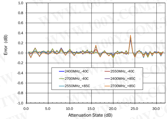
Successive Step Error versus Attenuation State
