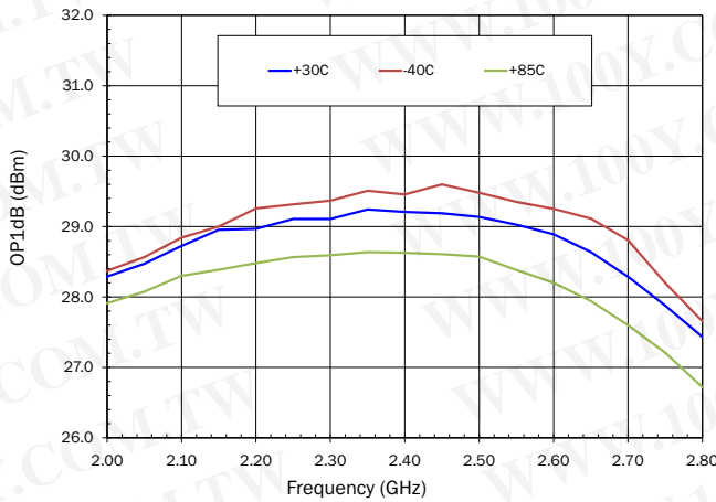
Output P1dB versus Frequency
