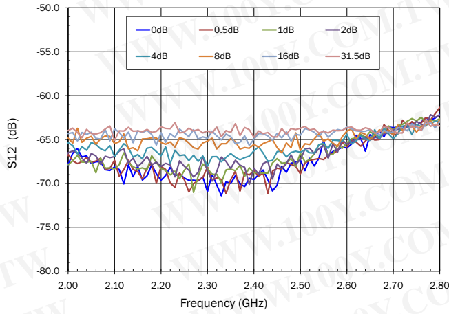
Isolation versus Frequency
