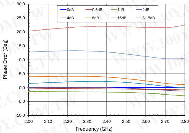
Normalized Phase Error versus Frequency
