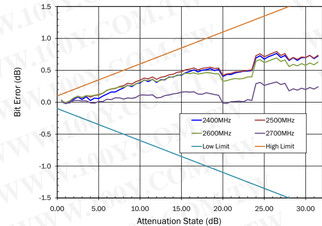
Bit Error versus Attenuation State
