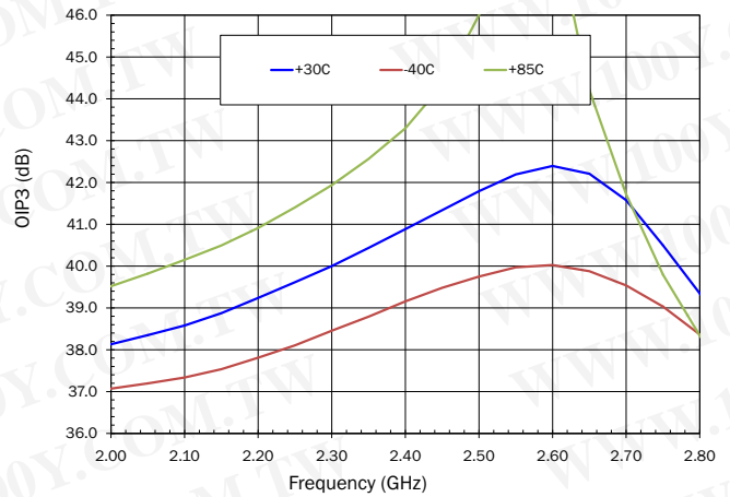
Output IP3 versus Frequency
