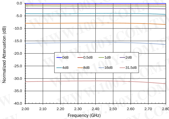
Normalized Attenuation versus Frequency
