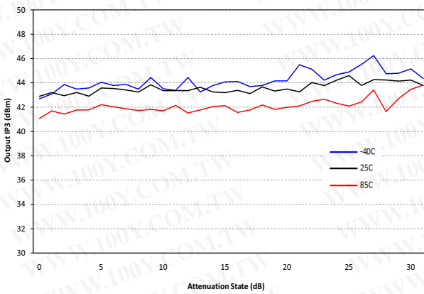
Output IP3 (dBm) versus Attenuation at 180MHz, P OUT 5dBm/Tone
