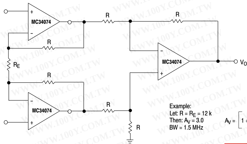
Figure 62. High Impedance Differential Amplifier
