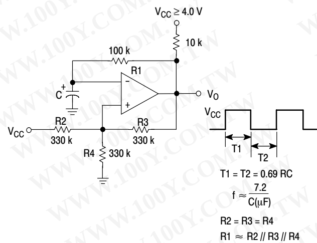
Figure 8. Squarewave Oscillator
