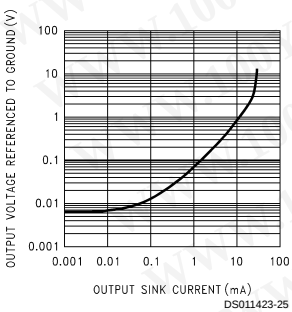
Output Characteristics Sinking Current
