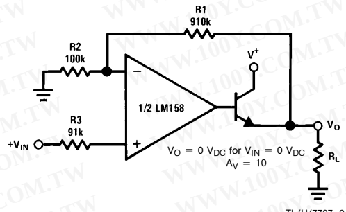
Power Amplifier
