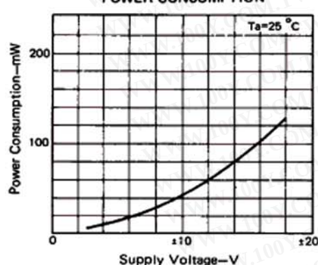
POWER CONSUMPTION
