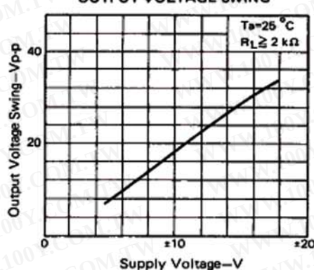
OUTPUT VOLTAGE SWING
