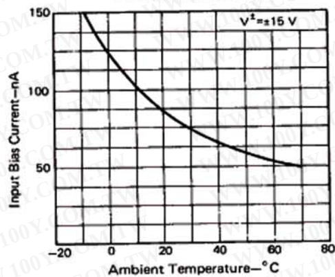
INPUT BIAS CURRENT
