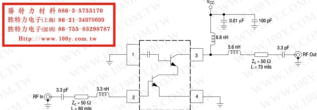
Figure 3. 1.9 GHz Application Configuration Circuit
