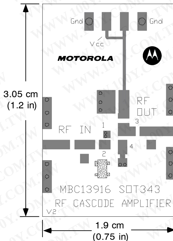
Figure 2. 900 MHz Printed Circuit Board
