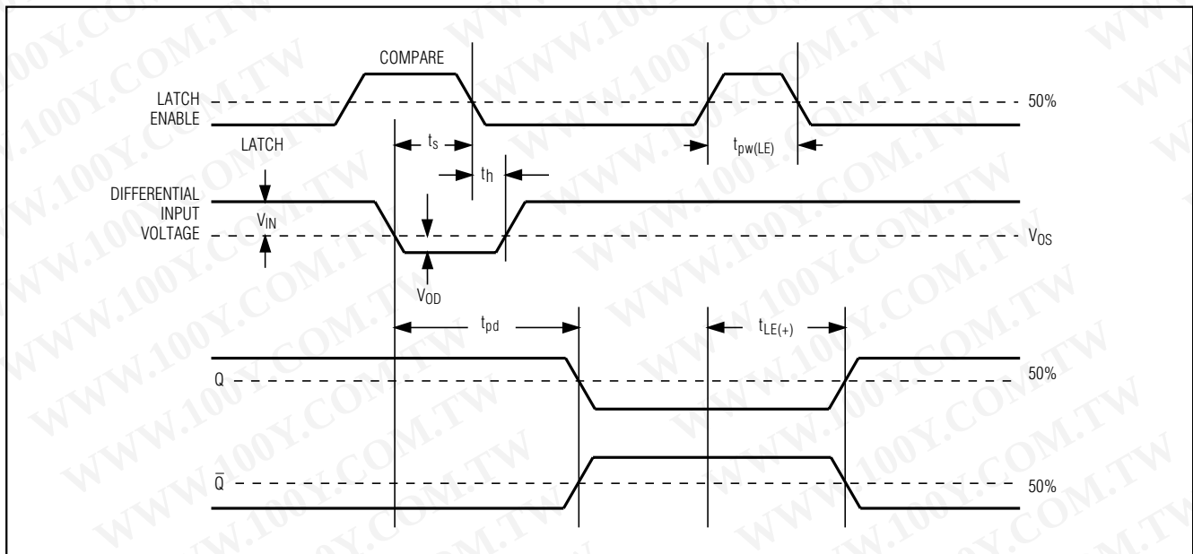
Figure 3. Timing Diagram
