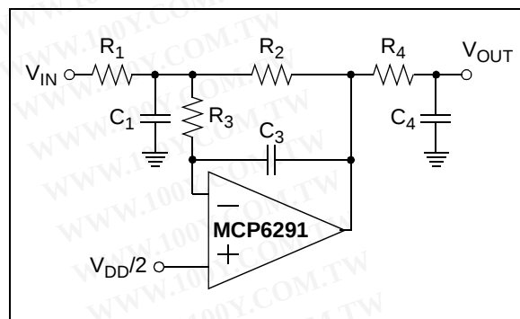
FIGURE 4-7: Multiple Feedback Low-Pass Filter.
