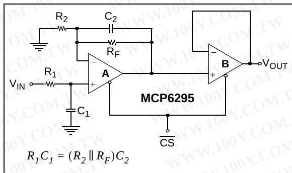
FIGURE 4-12: Buffered Non-Inverting Integrator with Chip Select.
