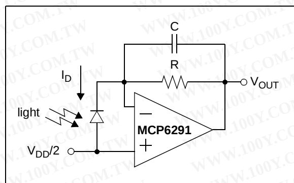
FIGURE 4-8: Photodiode Amplifier.
