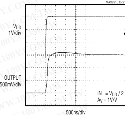
POWER-UP SETTLING TIME
