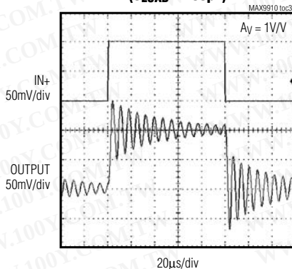
OUTPUT WAVEFORM WITHOUT R_{ISO} ( C_{LOAD} = 100pF )
