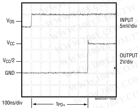
PROPAGATION DELAY t_{PD+} LOW-POWER MODE ( V_{CC} = +5V )
