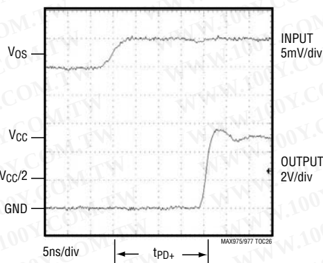
PROPAGATION DELAY t_{PD+} HIGH-SPEED MODE ( V_{CC} = +5V )
