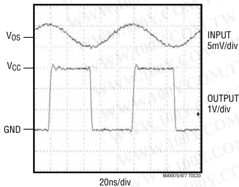
10MHz RESPONSE HIGH-SPEED MODE ( V_{CC} = +3V )
