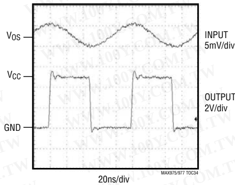
10MHz RESPONSE HIGH-SPEED MODE ( V_{CC} = +5V )
