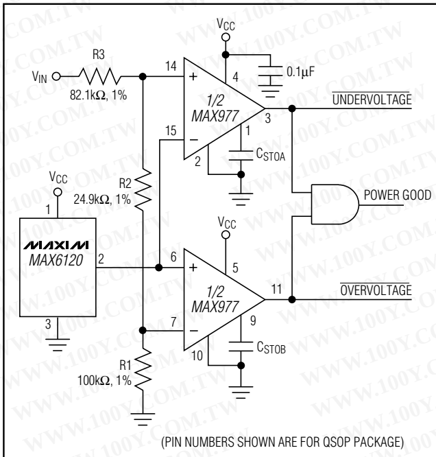
Figure 5. Window Comparator
