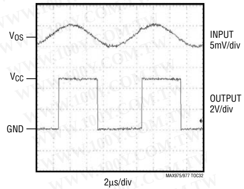
100kHz RESPONSE LOW-POWER MODE ( V_{CC} = +5V )
