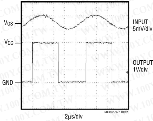
100kHz RESPONSE LOW-POWER MODE ( V_{CC} = +3V )
