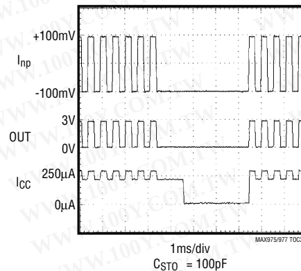
MAX975 AUTO-STANDBY OPERATION
