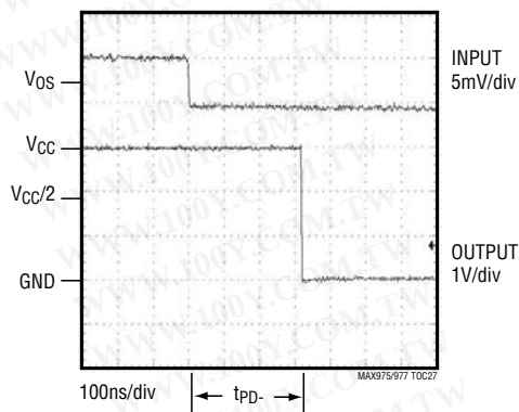
PROPAGATION DELAY t_{PD-} LOW-POWER MODE ( V_{CC} = +3V )
