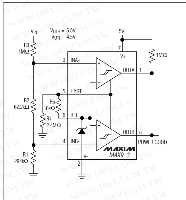
Figure 5. Window Detector
