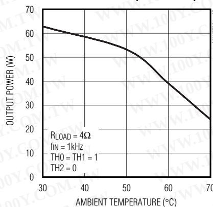
MAXIMUM STEADY-STATE OUTPUT POWER vs. TEMPERATURE (MONO MODE)*
