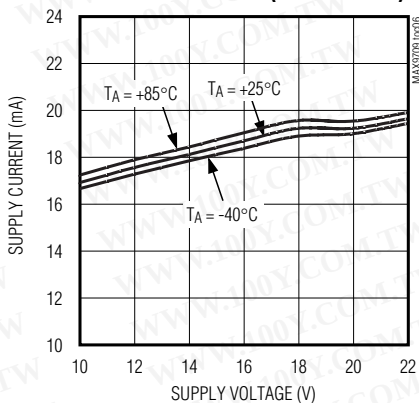
NO-LOAD SUPPLY CURRENT vs. SUPPLY VOLTAGE (STEREO MODE)
