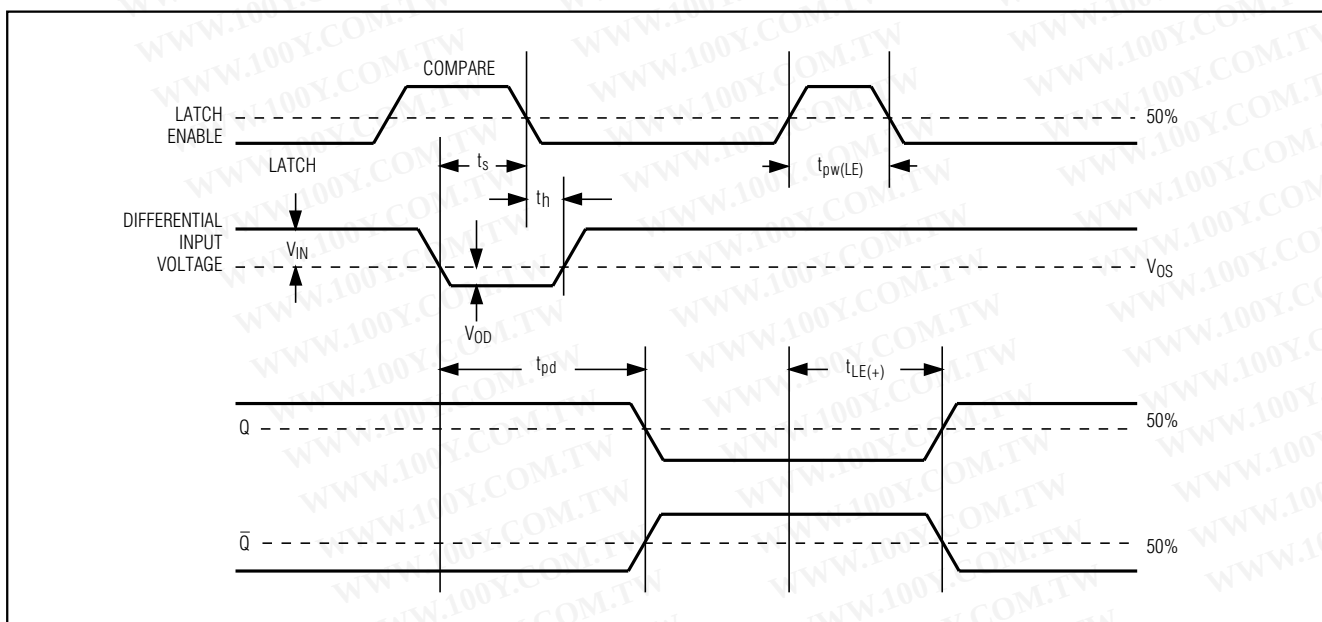
Figure 3. Timing Diagram
