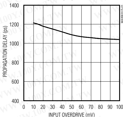
WORST-CASE PROPAGATION DELAY vs. INPUT OVERDRIVE
