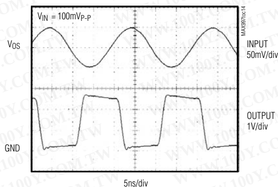
50MHz RESPONSE
