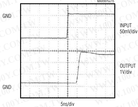
PROPAGATION DELAY (t PD+ )
