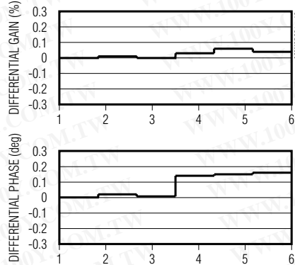
MAX9503G DIFFERENTIAL GAIN AND PHASE
