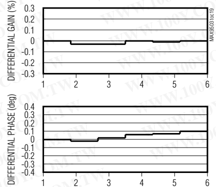
MAX9503M DIFFERENTIAL GAIN AND PHASE
