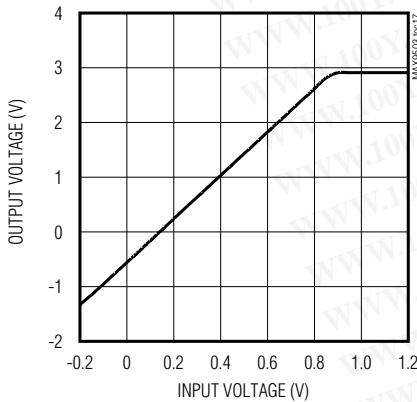
MAX9503M OUTPUT VOLTAGE vs. INPUT VOLTAGE
